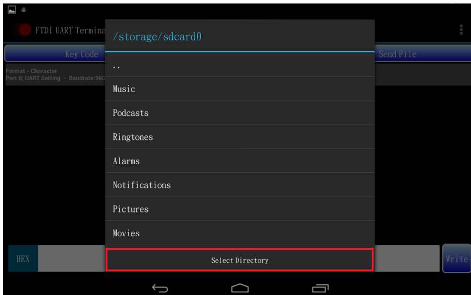
Figure 12 Select Directory
