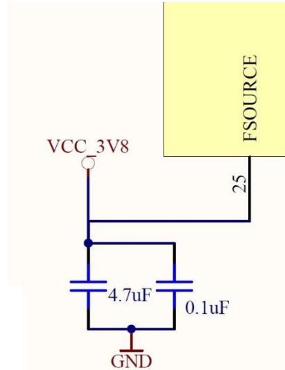
Figure 7-7 FSOURCE for eFUSE
