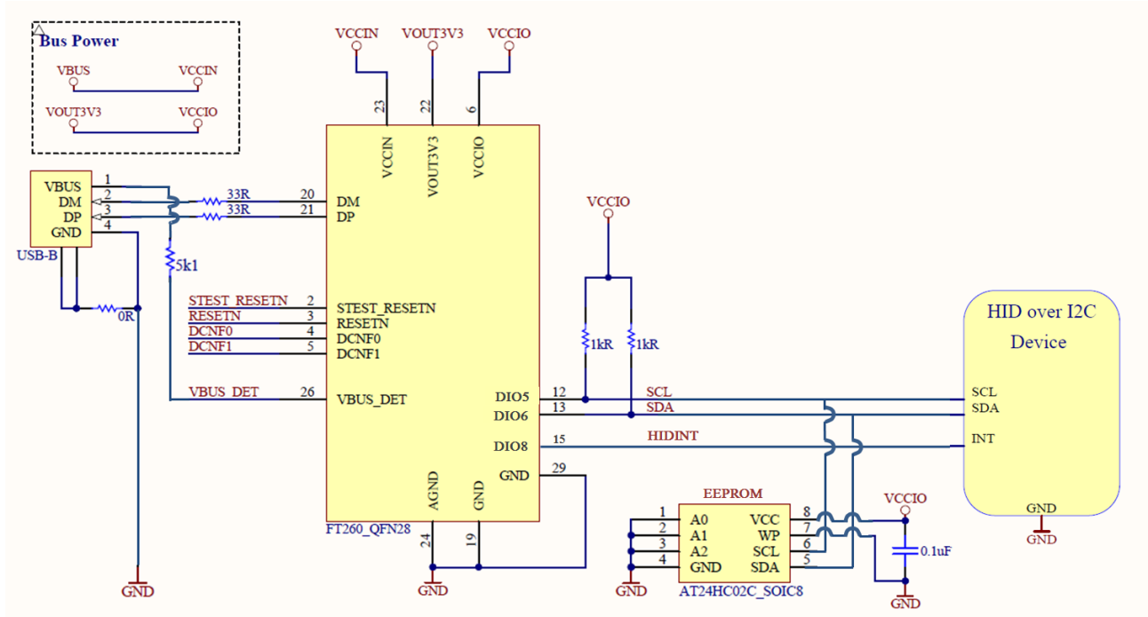
Figure 8-1 Application Example 1: HID over I 2 C
